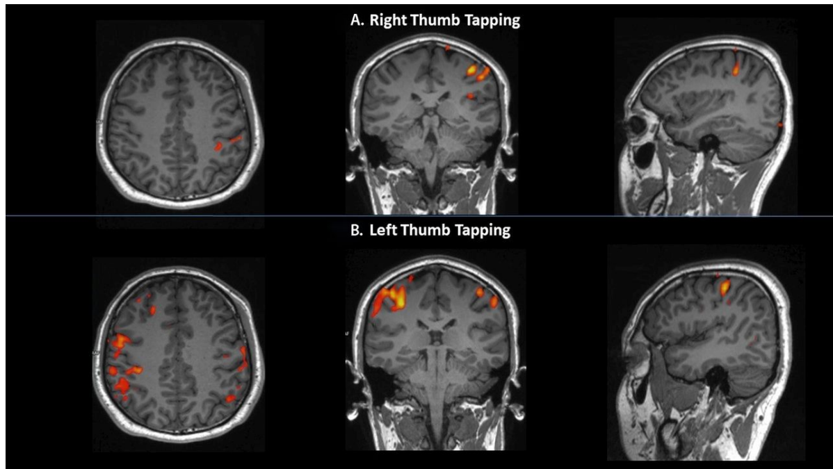
Fig. 2.2: Localised neurons during right- and left-thumb movement using functional magnetic resonance imaging (fMRI; Rashid et al., 2018 ).
