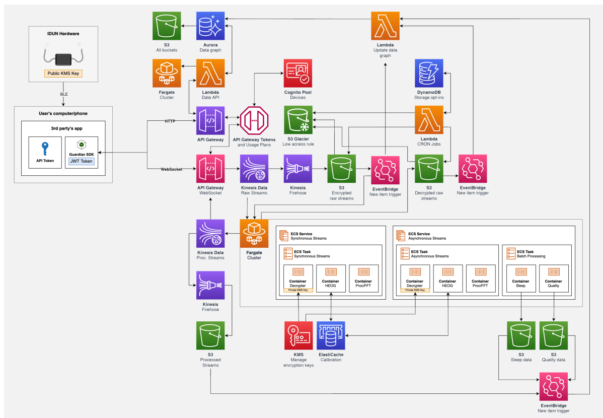
Fig. 5.7: Implementation architecture of IDUN's N/CI.
