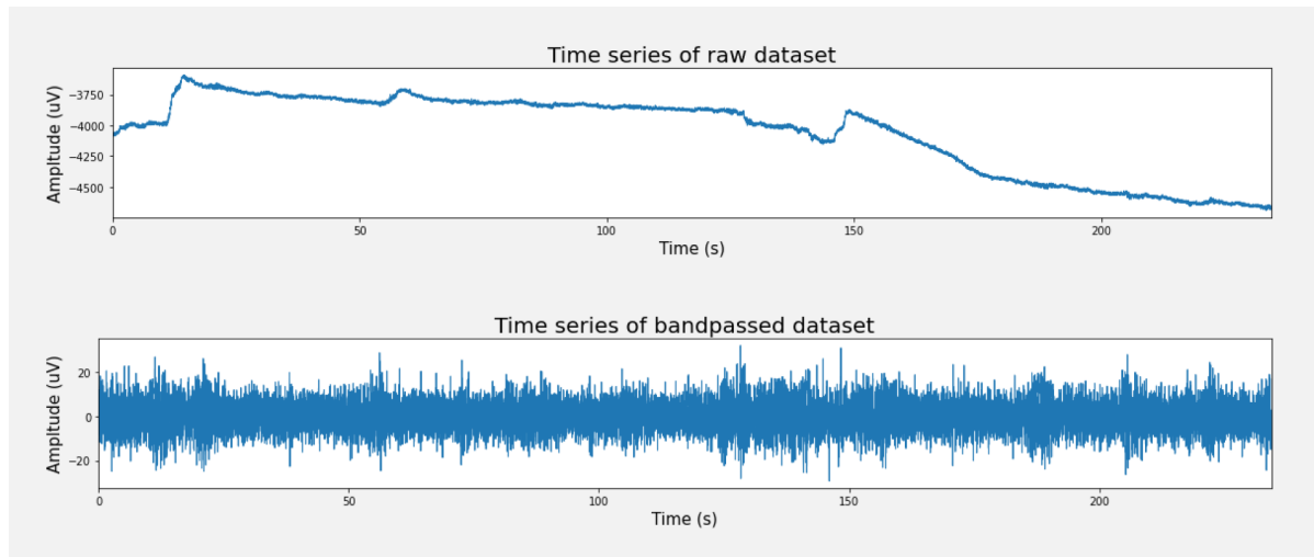
Fig. 3.1: Difference between raw and filtered data from IDUN's product.
