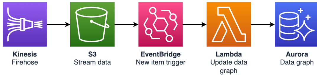
Fig. 5.9: The initial data flow in IDUN's N/CI.
