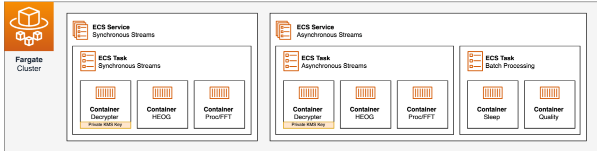
Fig. 5.8: The Fargate cluster of the example architecture for IDUN's N/CI.
