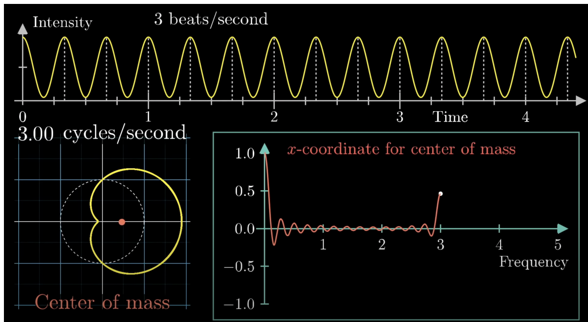
Fig. 5.1: Illustration of how FFT works (3Blue1Brown, 2018)
