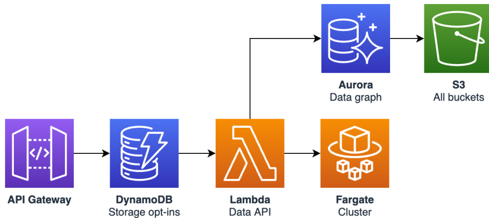
Fig. 5.12: API access part of the architecture of IDUN's N/CI.
